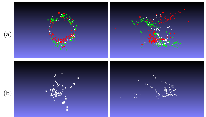
Fig. 14 Front views (left) and side views (right) of the 3-D reconstruction from the data set in Fig.13. (a) Using the three frames. (b) Using the 1st-2nd frame pair. Reconstruction from the 0th-1st frame pair and reconstruction from the 0th-2nd frame pair both fail.
