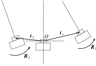
Fig. 3 The translations \mathbf{t}_1 and \mathbf{t}_2 and the rotations \mathbf{R}_1 and \mathbf{R}_2 of the 1st and 2nd cameras relative to the 0th camera.
