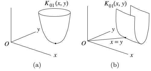
Fig. 4 (a) The values of x and y minimize K_{01}(x, y) , and the minimum is 0. (b) For a fixing camera configuration, the minimum of K_{0,1}(x, y) is not uniquely determined. If x = y , the solution is at the intersection of the minimum contour of K_{0,1}(x, y) with the line x = y .
